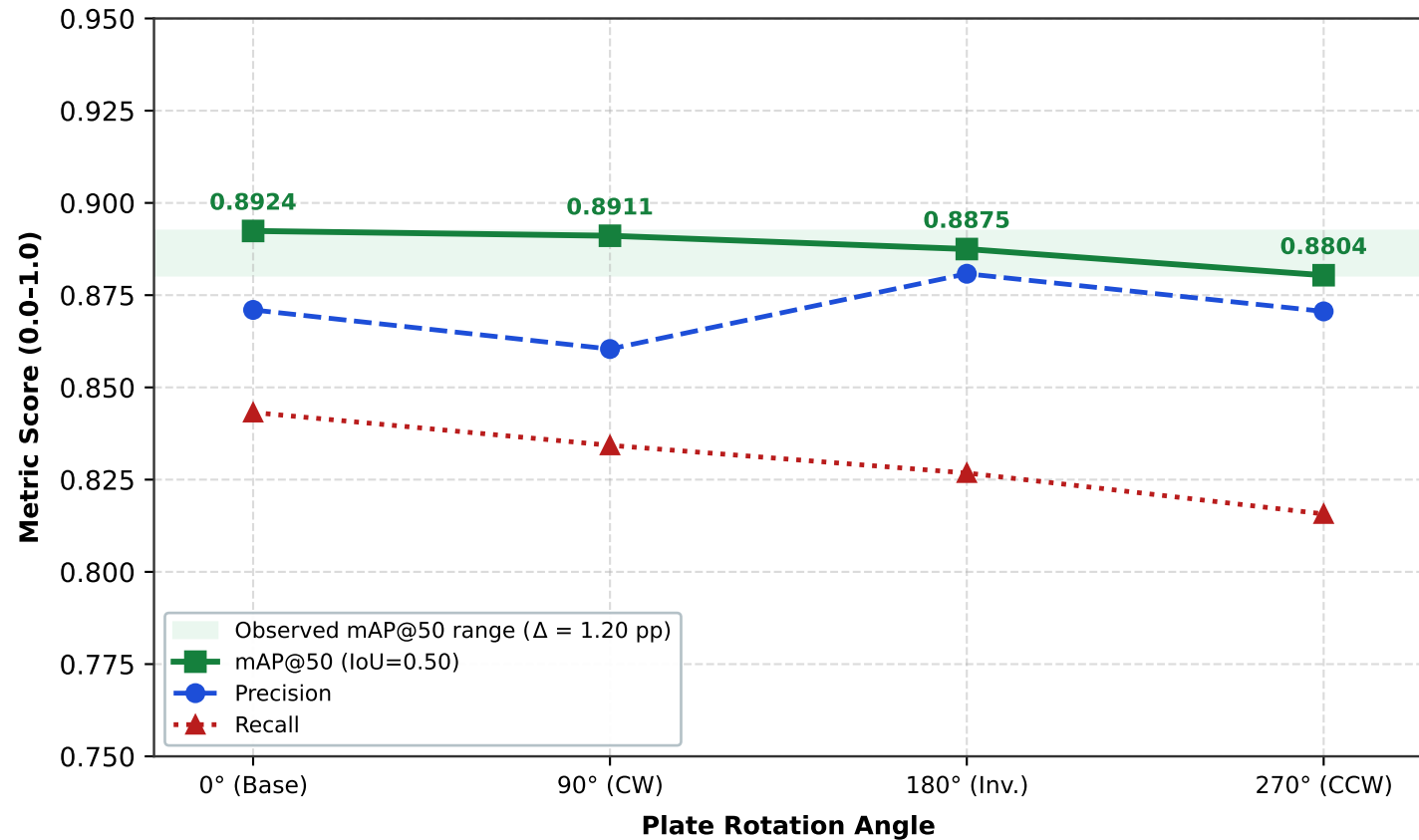
(b) Rotational Invariance Robustness (N=200 Plate Images)
